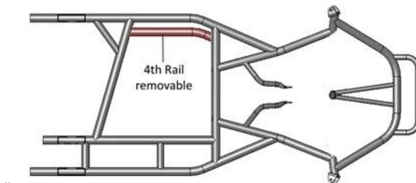
24. Chassis diagram.
